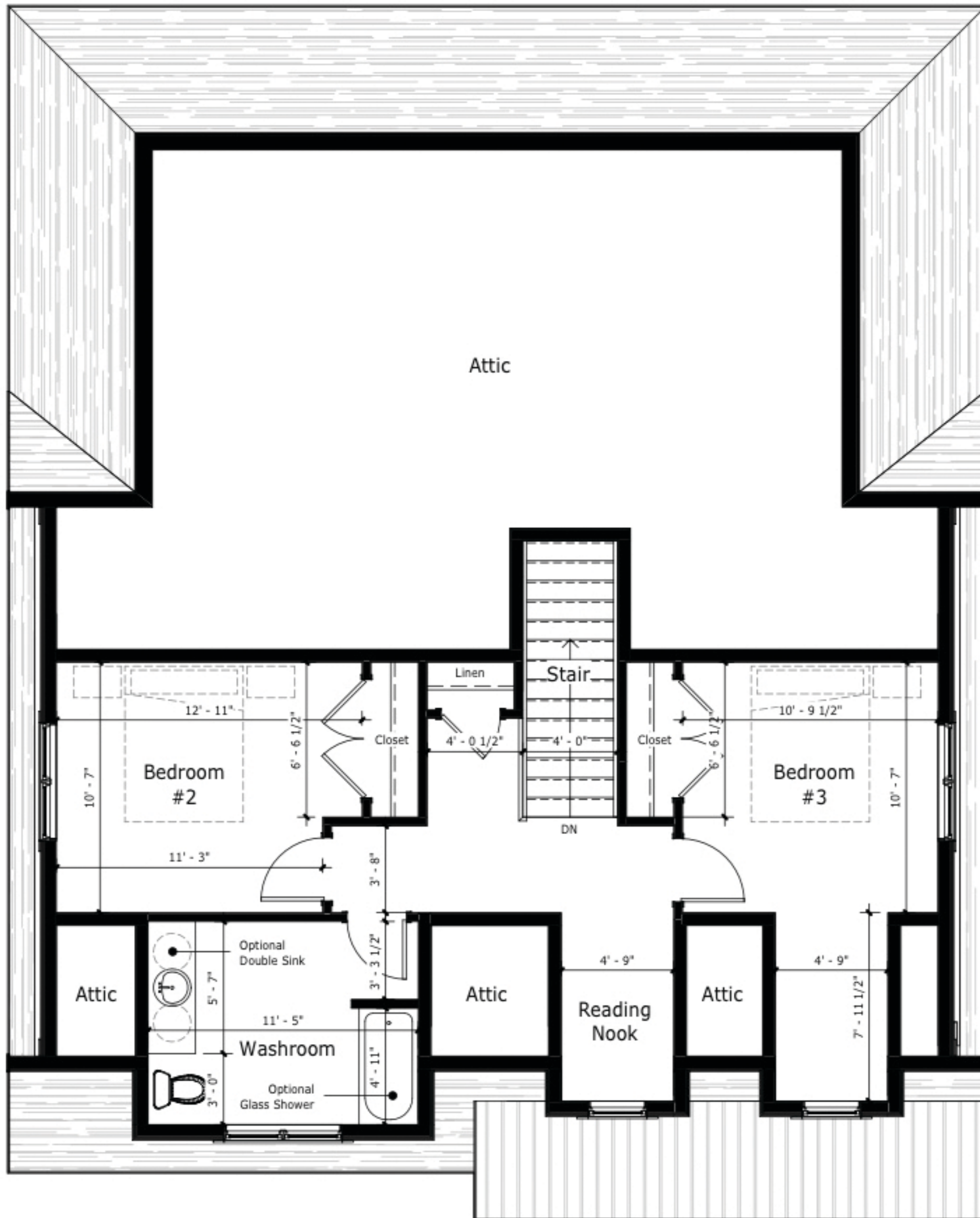
Second Floor Plan 3/16" = 1'-0"
